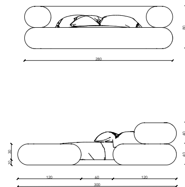
Plan & elevations
